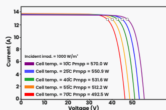
IV Curve Variation with Temperature
